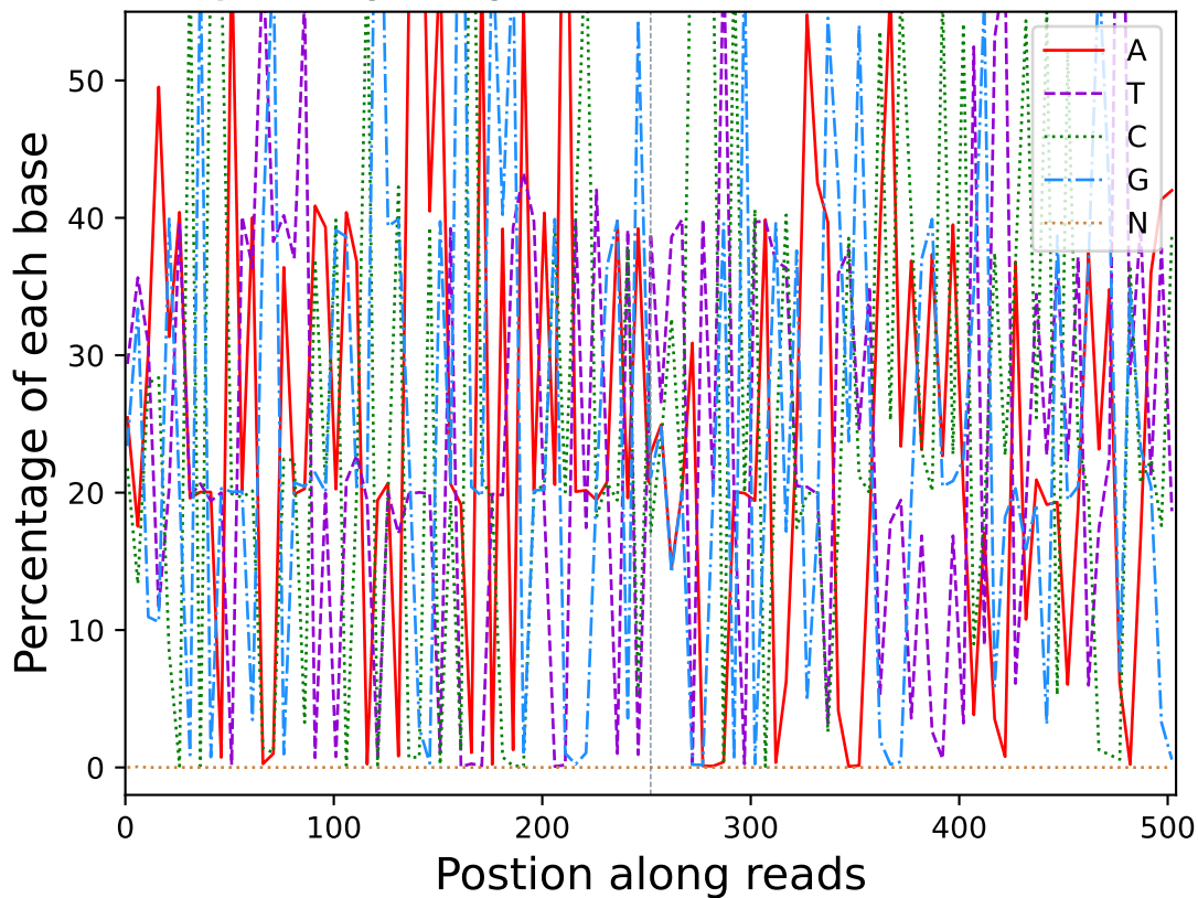
Base percentage along reads (R10217)
